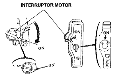
INTERRUPTOR MOTOR
